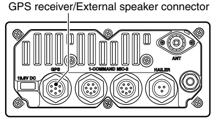
Transceiver's rear panel
